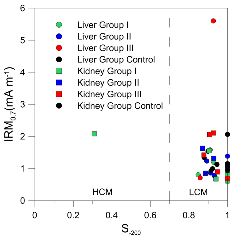
Figure 4. Relationship between S_{-200} and measures of IRM_{0.7} for all liver (circles) and kidney (square) samples.
