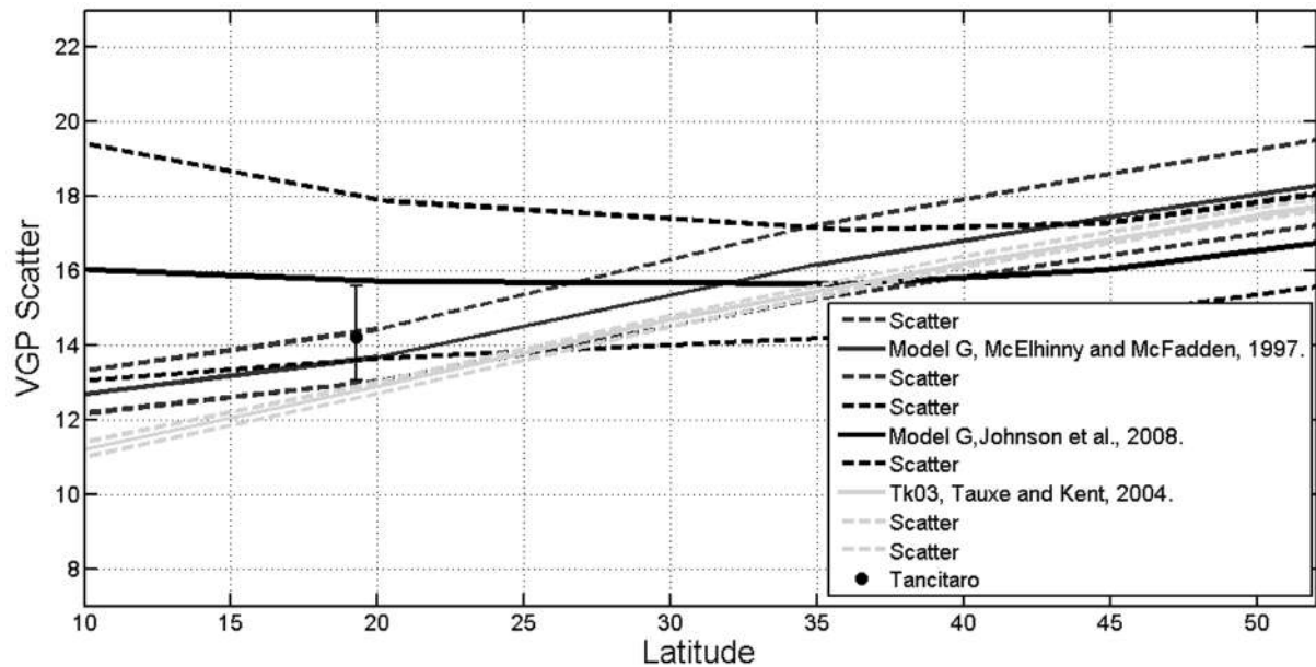
Figure 7. Scatter of the VGP as a function of the latitude for the last 5 Myr, compared with the curves of reference provided by the Model G proposed by McElhinny and McFadden (1997) and Johnson et al. (2008), also with the Tk03.GAD model of Tauxe and Kent (2004).
