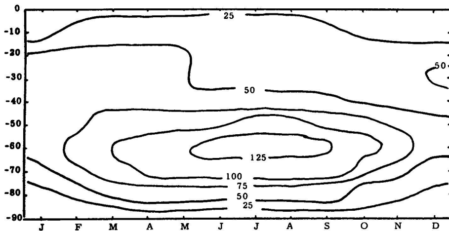
Figure 5. As Fig. 4, but for 25 cb.
