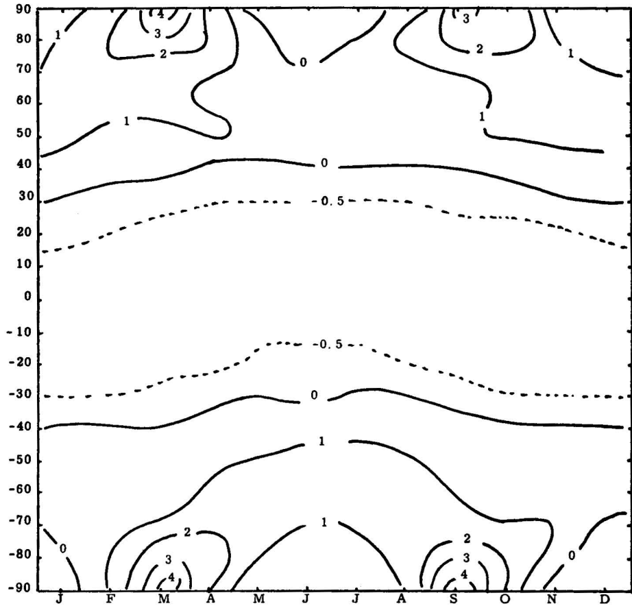
Figure 12. As Fig. 6, but for Exp. No. 2.
