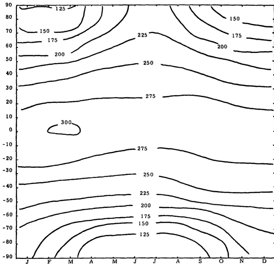
Figure 3. The computed 50 cb temperatures as a function of latitude and time. Unit: °K.
