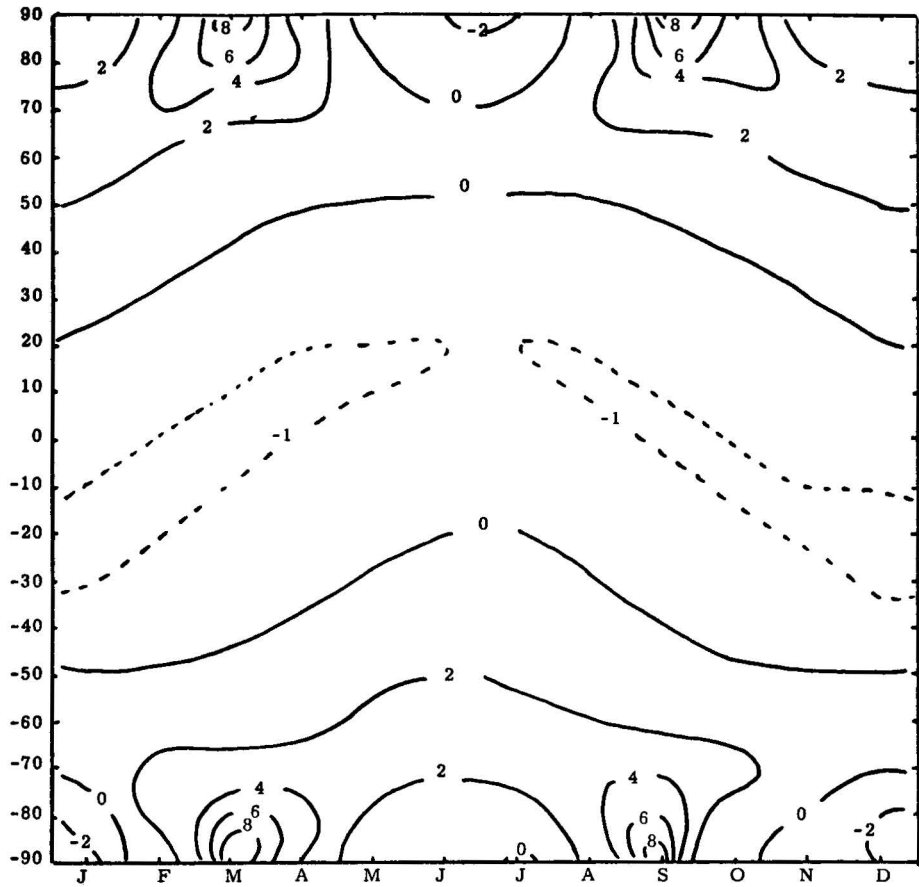
Figure 11. As Fig. 6, but for Exp. No. 1.
