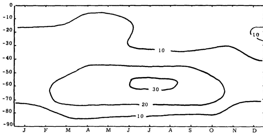
Figure 4. The zonally averaged winds at the 75cb level as a function of latitude and time. Unit: \text{msec}^{-1} .
