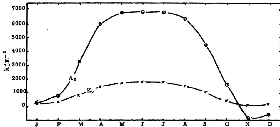
Figure 17. As Fig. 7, but for Exp. No. 1.
