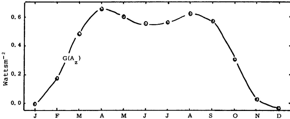
Figure 19. As Fig. 8, but for Exp. No. 1.
