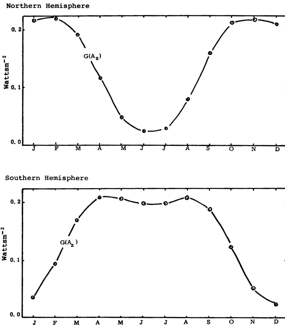
Figure 20. As Fig. 8, but for Exp. No. 2.
