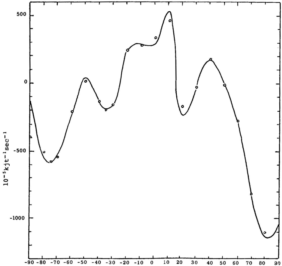
Figure 2. The heating for January as a function of latitude. Solid curve is the deviation H from the average over the globe. The circles are the points, obtained by summing the series of Legendre polynomials with N = 17 . Unit: 10^{-5} \text{ kJt}^{-1} \text{ sec}^{-1} .
