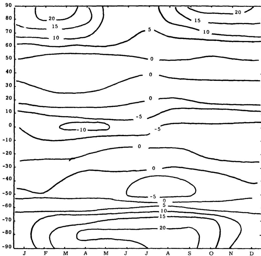
Figure 6. The zonally averaged vertical velocity as a function of latitude and time. Unit: 10^{-6} \text{ cbsec}^{-1} .
