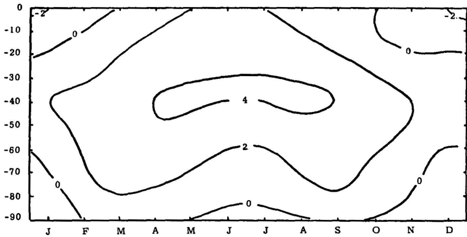
Figure 14. As Fig. 4, but for Exp. No. 2.
