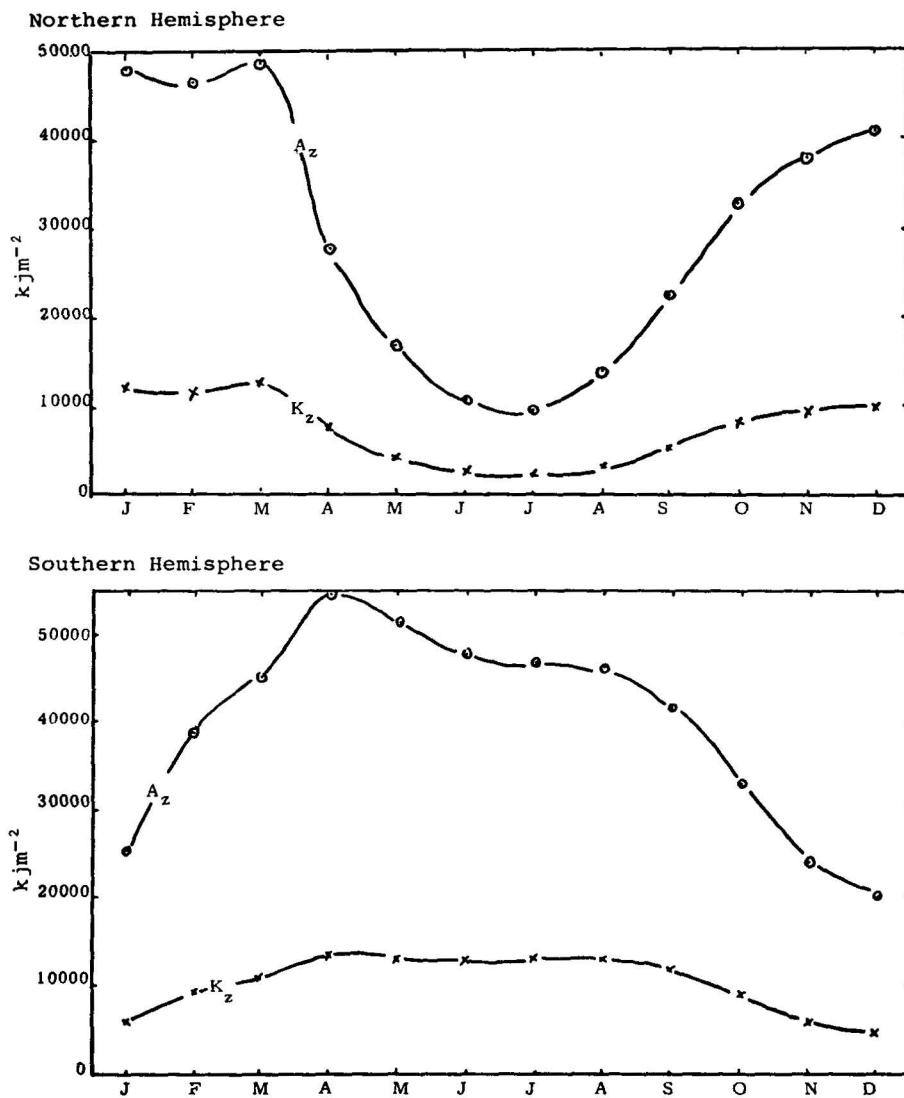
Figure 7. Available potential and kinetic energy as a function of time. Unit: \text{kJ m}^{-2} .
