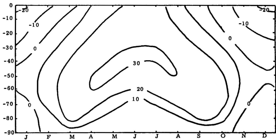
Figure 15. As Fig. 5, but for Exp. No. 1.
