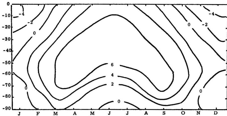
Figure 13. As fig. 4, but for Exp. No. 1.
