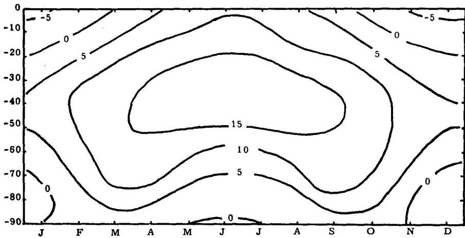
Figure 16. As Fig. 5, but for Exp. No. 2.
