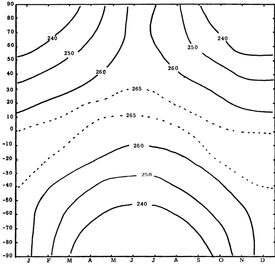
Figure 10. As Fig. 3, but for Exp. No. 2.
