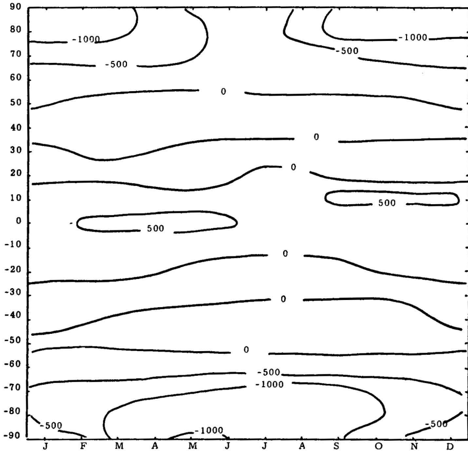
Figure 1. The heating of an atmospheric column as a function of latitude and time. Unit: 10^{-5} \text{ kJt}^{-1} \text{ sec}^{-1} (Fuenzalida, 1973).
