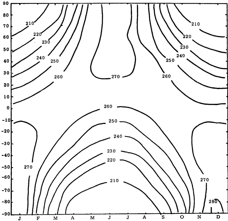
Figure 9. As Fig. 3, but for Exp. No. 1.
