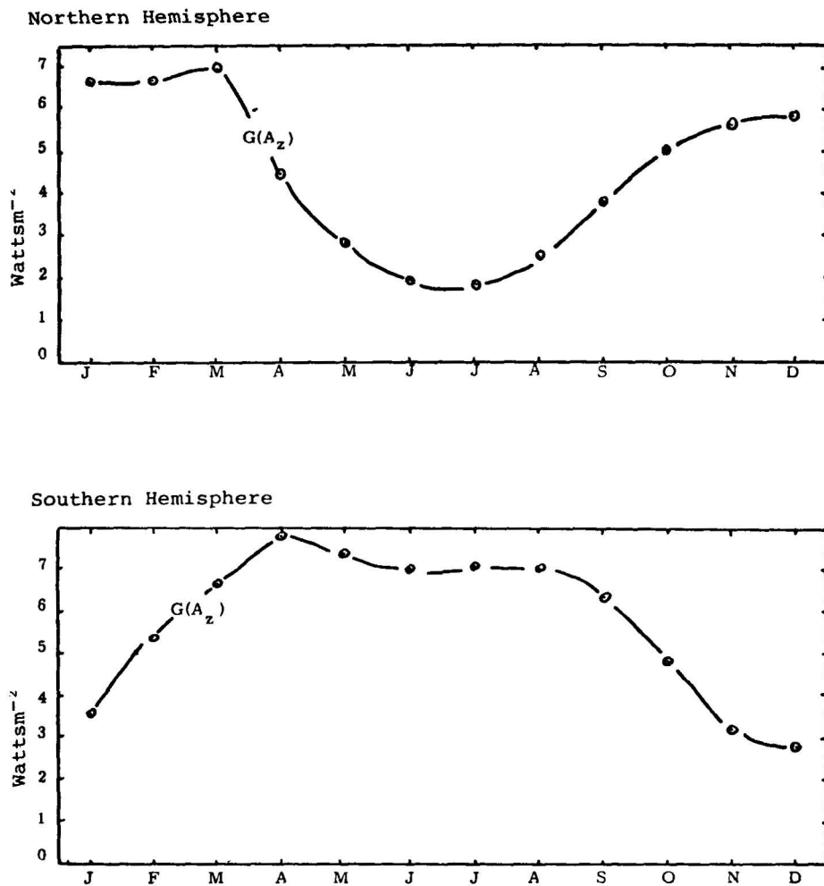
Figure 8. The generation of available potential energy as a function of time. Unit: Wattsm -2 .
