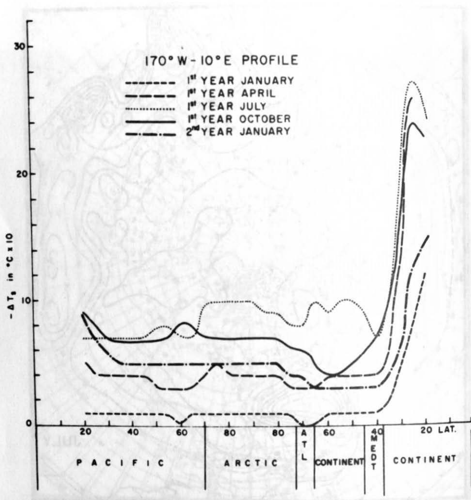
Fig. 2. The negative of the anomalies of surface temperature, in tenths of Celsius degrees, along the transpolar longitudes 170^{\circ} \text{ W} - 10^{\circ} \text{ E} , due to a decrease of two percent in the solar constant, for different periods of integration. The short dashed line represents the January values after a single time step of one month; the long dashed line, the April values after four months, the dotted line, the July values after seven months; the dotted line, the July values after seven months, the continuous line, the October values after ten months and the dotted-dashed line represents the January values after thirteen months.
