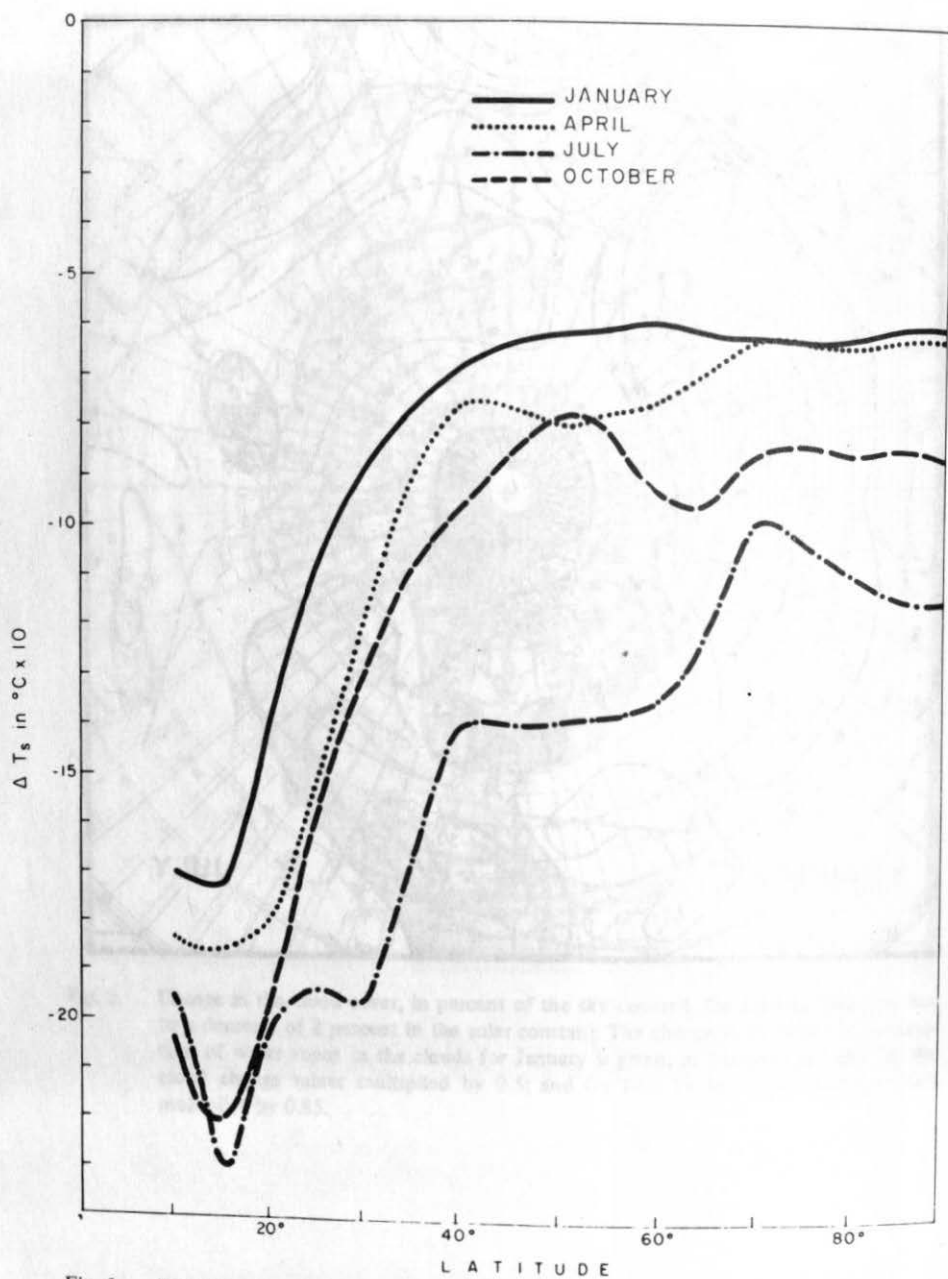
Fig. 6. Zonally averaged values of the change in the surface temperature, in tenths of degrees Celsius, due to a decrease of 2 percent in the solar constant.
