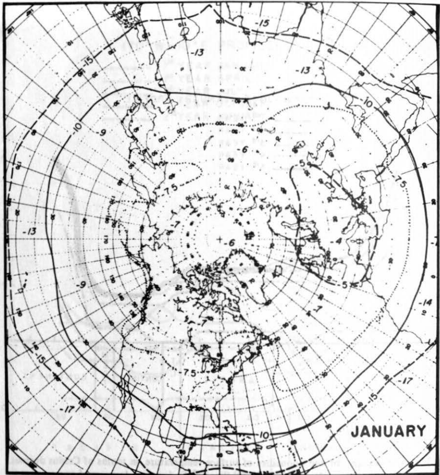
Fig. 4. Change in mid-tropospheric temperature in January and July, in tenths of Celsius degrees, due to a decrease of 2 percent in the solar constant.
