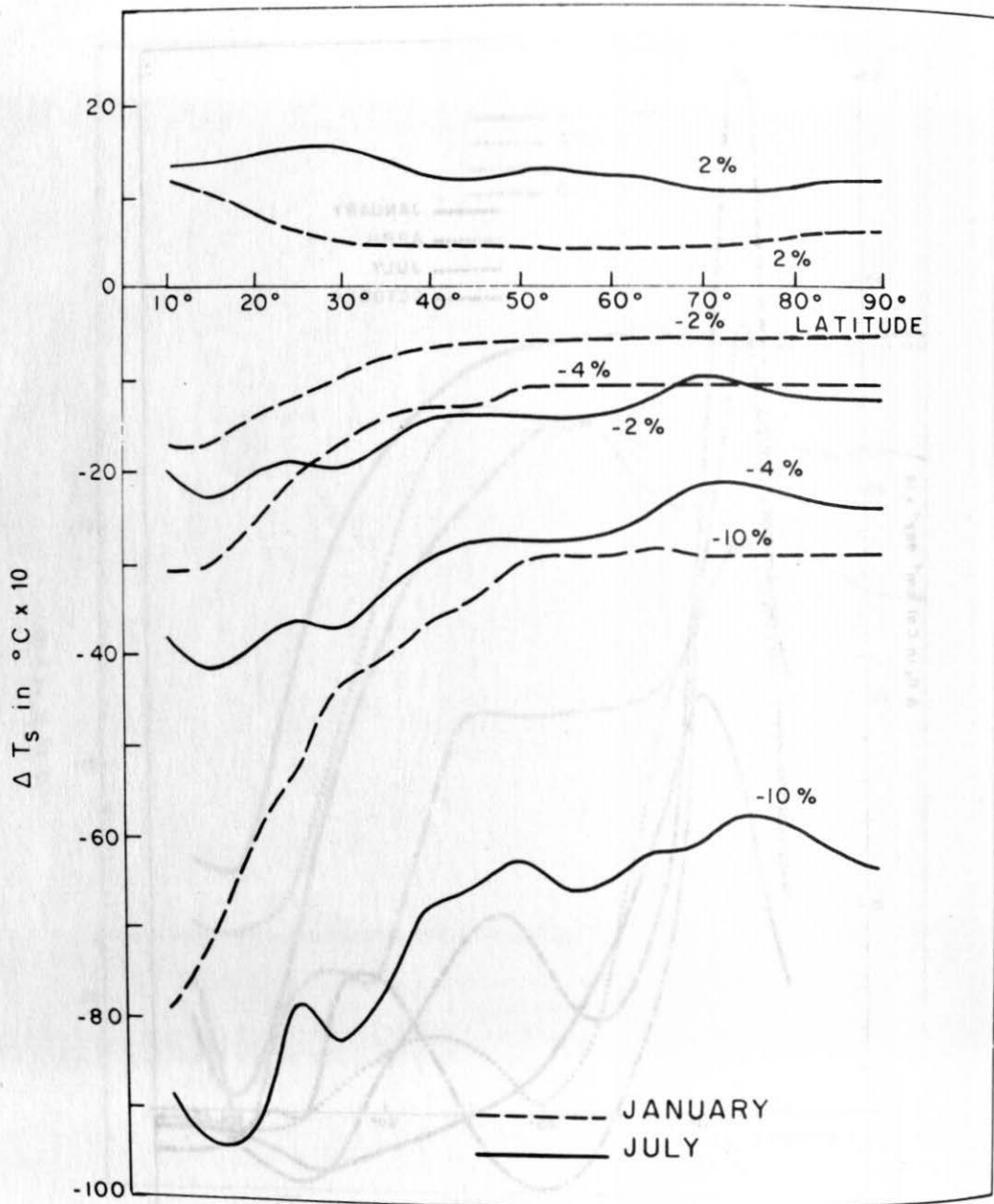
Fig. 8. Zonally averaged values of surface temperature change, in tenths of Celsius degrees, for January and July, corresponding to changes of the solar constant of +2, -2, -4 and -10 percent.
