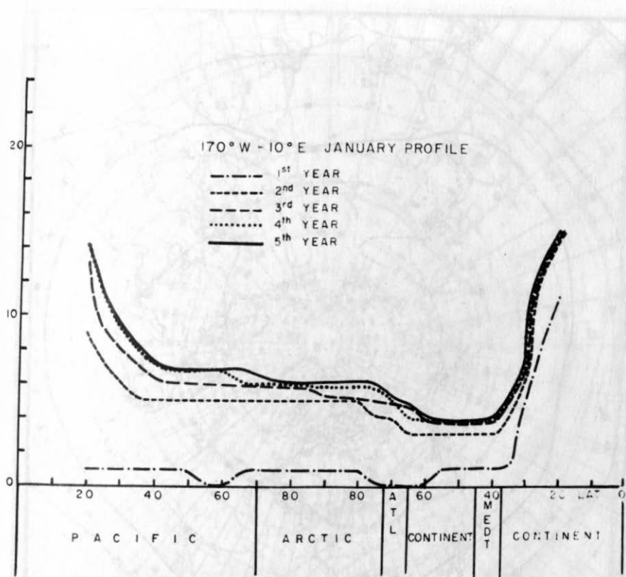
Fig. 3. The negative of the anomalies of surface temperature, in tenths of Celsius degrees, along the transpolar longitude 170^{\circ} \text{ W} - 10^{\circ} \text{ E} , due to a decrease of two percent in the solar constant, for January and for different periods of integration. The dotted-dashed line represents the values after a single time step of one month; the short dashed line, the values after thirteen months; the long dashed line, after 25 months; the dotted line, after 37 months, and the continuous line represents the values after 49 months.
