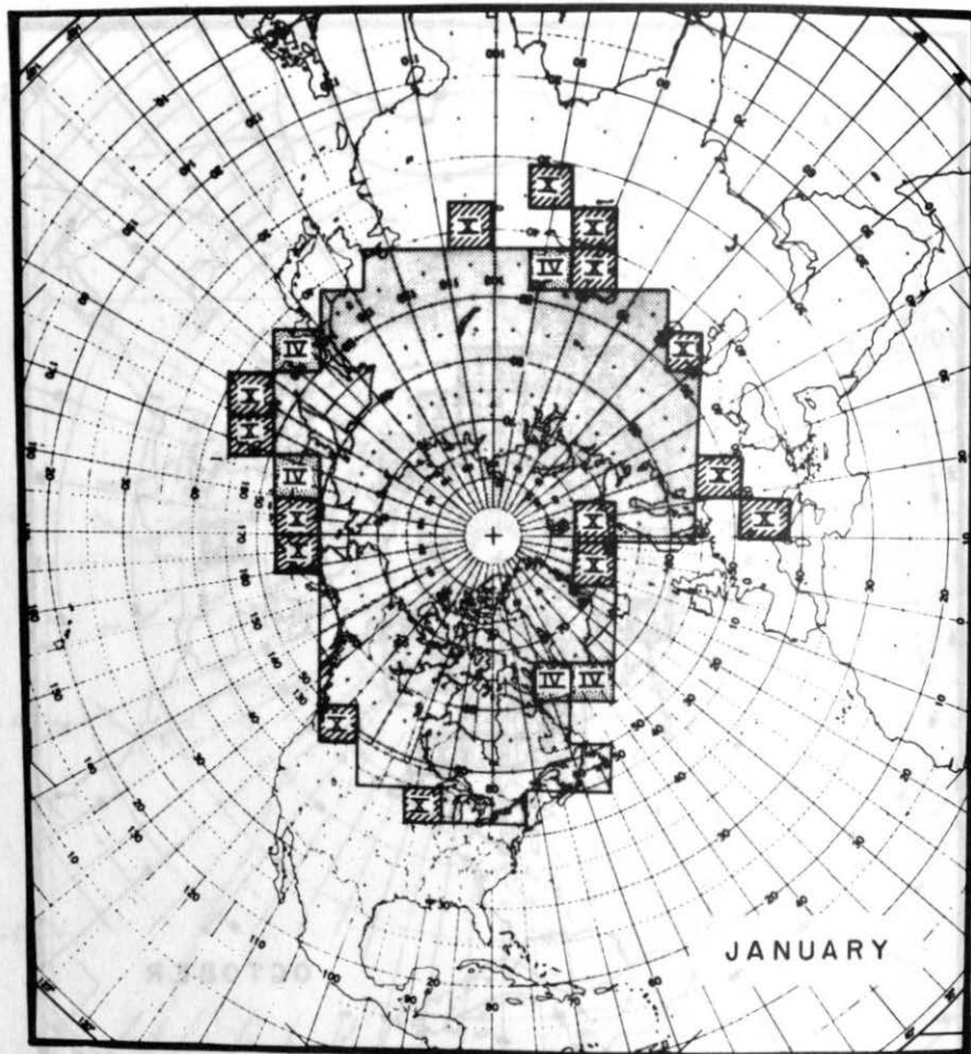
Fig. 10. Snow and ice cover generated by the model in January for different values of the solar constant. The closed region around the pole correspond to present normal conditions; the squares labeled IV are the increases due to a decrease of 4 percent in the present value; and those labeled IV and X are the increases due to a decrease of 10 percent.
