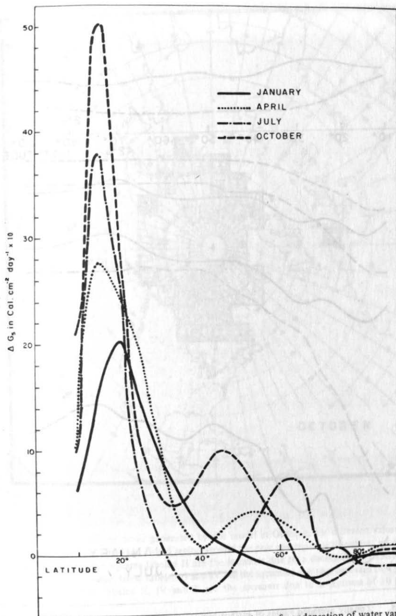
Fig. 7. Zonally averaged values of the change in the heat of condensation of water vapor in the clouds, in tenths of Langleys per day, due to a decrease of 2 percent in the solar constant.
