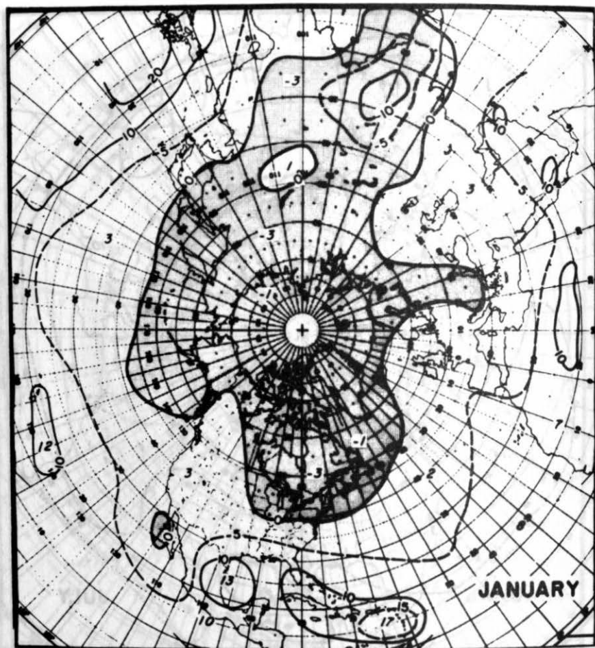
Fig. 5. Change in the cloud cover, in percent of the sky covered, for January and July due to a decrease of 2 percent in the solar constant. The change in the heat of condensation of water vapor in the clouds for January is given, in Langley's per day, by the cloud change values multiplied by 0.5; and for July by the corresponding values multiplied by 0.85.
