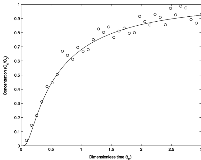
Fig. 1. Synthetic tracer breakthrough data obtained from the model for continuous injection (solid line) plus a Gaussian random noise (circles).
