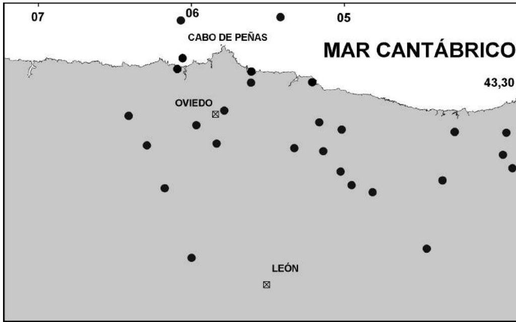
Fig. 10. Seismicity of Asturias. [Data provided by Instituto Geográfico Nacional. Black circles = epicenters.]
