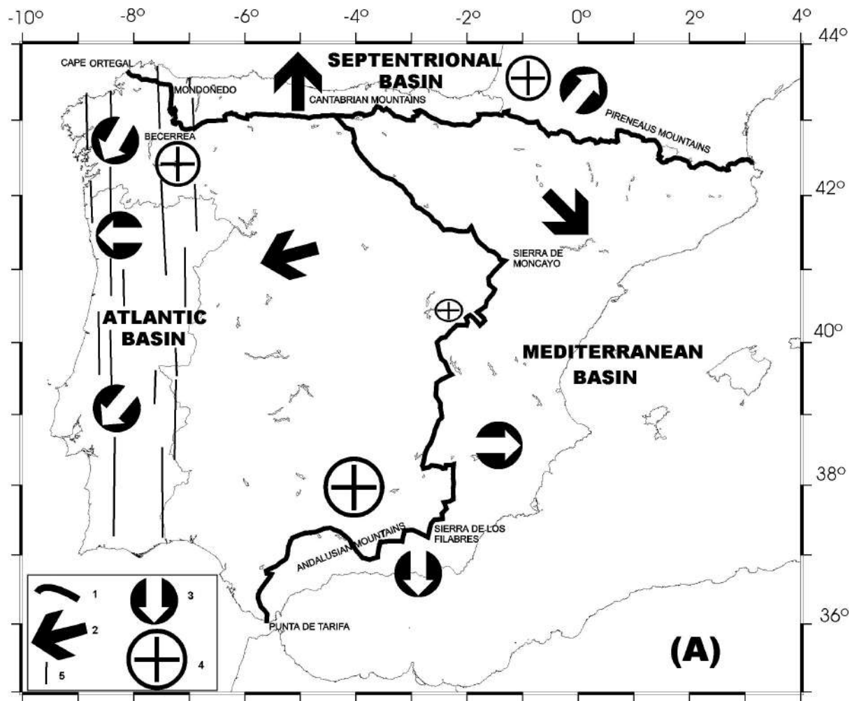
Fig. 5. Hydrographic characteristics of the Iberian Peninsula. [A) Fluvial network scheme of the Iberian Peninsula. 1: Principal Watershed; 2: main directions of the largest basins; 3: local directions of secondary basins; 4: rising zones; 5: selected alignments]; {B) Sketch of the main watersheds in Asturias. Continuous line = PPPO; discontinuous line = PPSO; black points = PPTO; largest basins: 1: north, 2: south; northern basins: A=Eo, B=Navia, C=Narcea-Nalón, D=Sella, E=Della}; {C) Scheme of IPEF data. 1: 0,1-0,29; 2: 0,3-0,49; 3: 0,5-0,69; 4: 0,7-0,79; 5: 0,8-0,95}; {D) Fluvial network of Asturias and surroundings. Rivers: 1=Eo, 2=Navia, 3=Narcea, 4=Nalón, 5=Sella.} See Table 10.]
