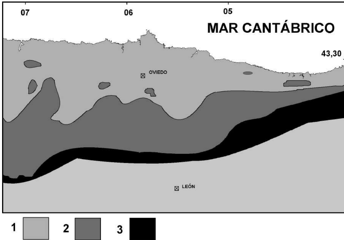
Fig. 13. Morphoisohips sketch of Asturias. [1: 0-1.000, 2: 1.000-1.500, 3: 1.500-2.000 (m)].
