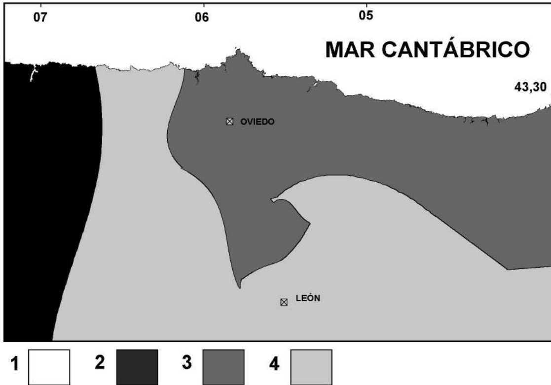
Fig. 17. Seismic zones of Asturias. [Mmax: 1- 5,5, 2- 5,3, 3- 5,0, 4- <5,0. See table 17.]
