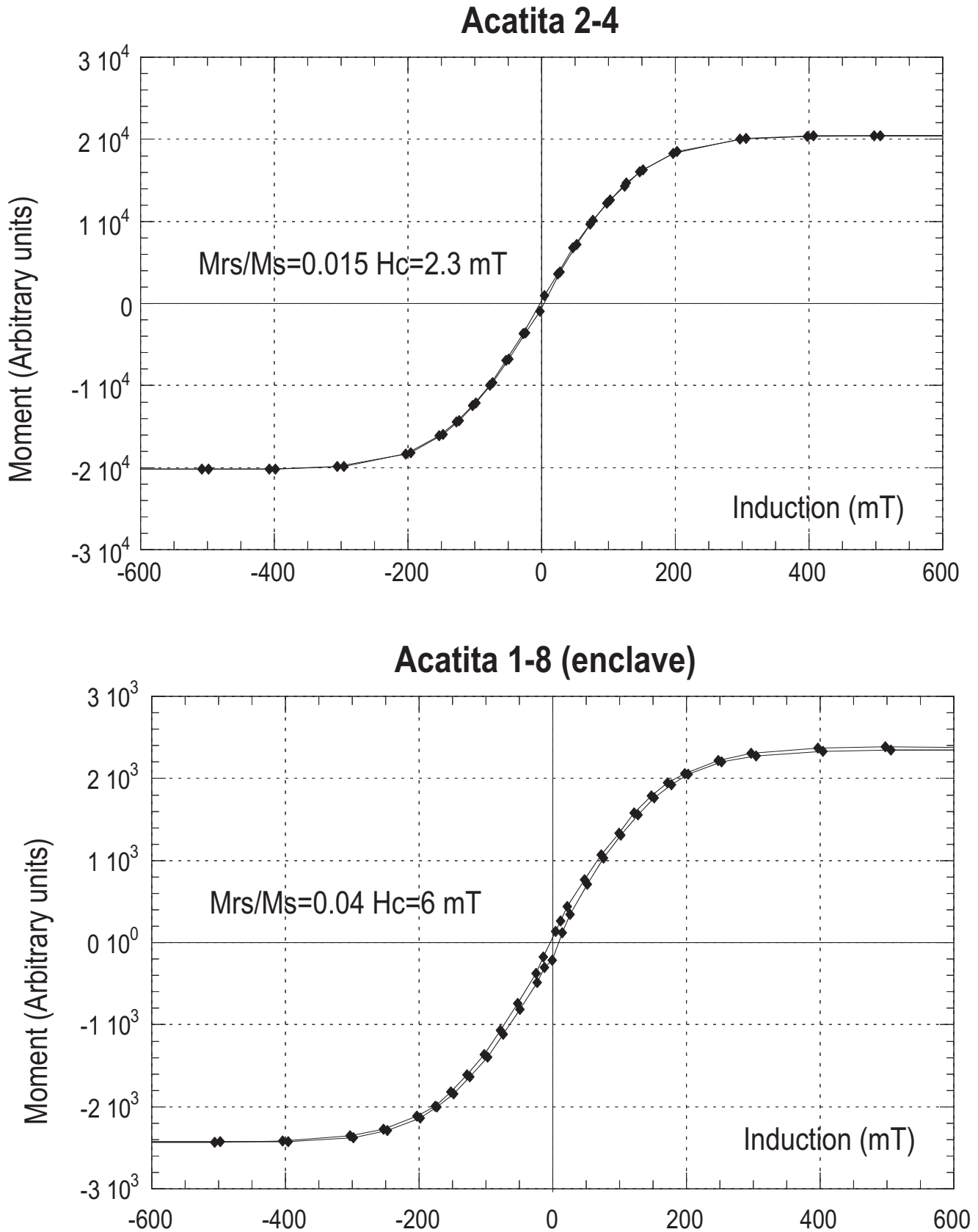
Fig. 5. Hysteresis curves for representative samples of the Acatita intrusions. Sample 1-8 is representative of the behavior observed in mafic enclaves, which generally have larger Mrs/Ms ratios than homogenous tonalite samples.
