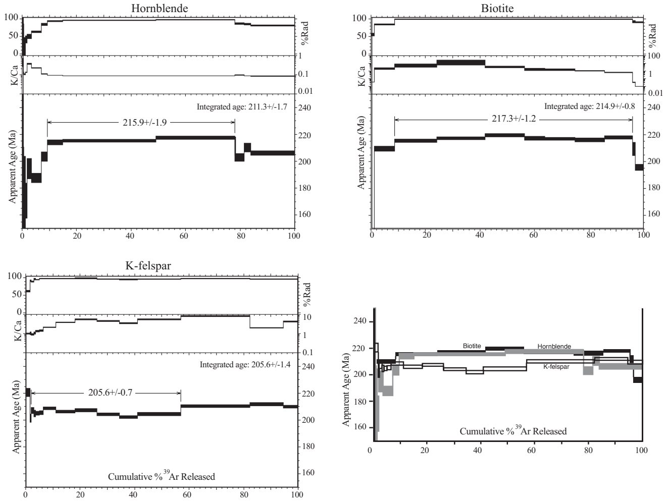
Fig. 3. 40 Ar/ 39 Ar apparent age spectra for biotite (a), hornblende (b), and K-feldspar (c) for a sample from the Acatita tonalite. Width of the horizontal bar on each diagram represents analytical error (1σ). The interval selected for age calculation is shown in each diagram.
