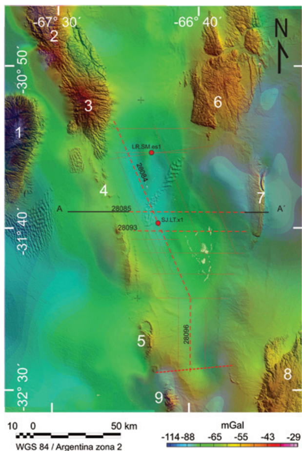
Fig. 9. Map of Bouguer Anomaly, superimposed with the digital elevation model of the terrain and location of the seismic lines reinterpreted (in dotted lines corresponding to Figs. 4, 5 & 6). Geological structures (ranges) are numerically identified as: 1- Pie de Palo, 2- Valle Fertil, 3- De la Huerta, 4- Guayaguas-Catanal, 5- Las Quijadas, 6- Chepes, 7- Ulapes, 8- San Luis, 9- Del Gigante. The profile identified as A-A' corresponds to the interpretation shown in Fig. 14.
