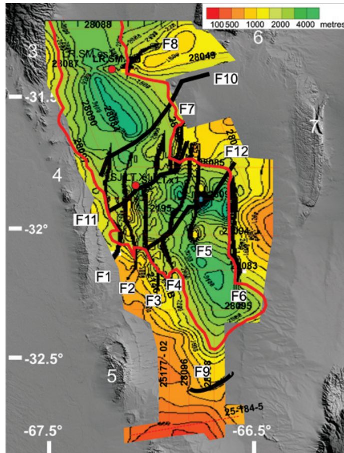
Fig. 7. Depth of the seismic basement in meters. Main geological structures (ranges): 3- De la Huerta, 4- Guayaguas-Catanal, 5- Las Quijadas, 6- Chepes, 7- Ulapes. Red line: basin limit, Red circles – Seismic Wells, Black wide line - identified geological faults as – F1, F2, F3, ..... F12, Soft red lines: seismic lines.
