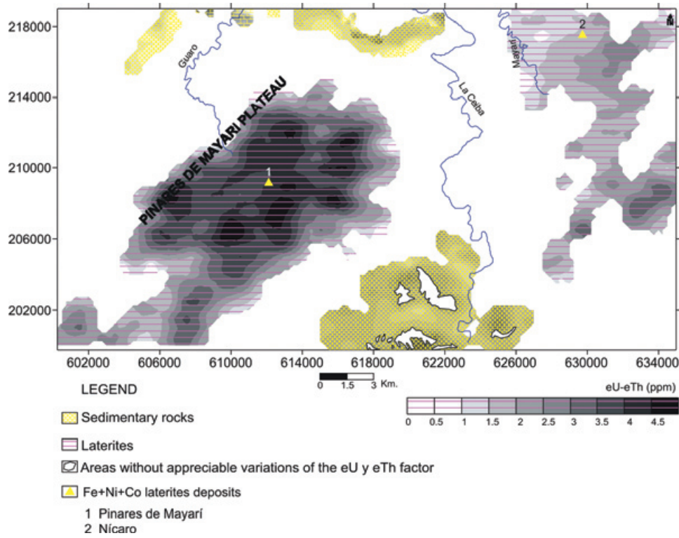
Fig. 10. Variations of the eU-eTh factor in the Mayarí sector. The increase of the gray color tonalities points out the qualitative valuation of the increase of thickness of the laterites crust and the increase in the clay grade of the sedimentary rocks.
