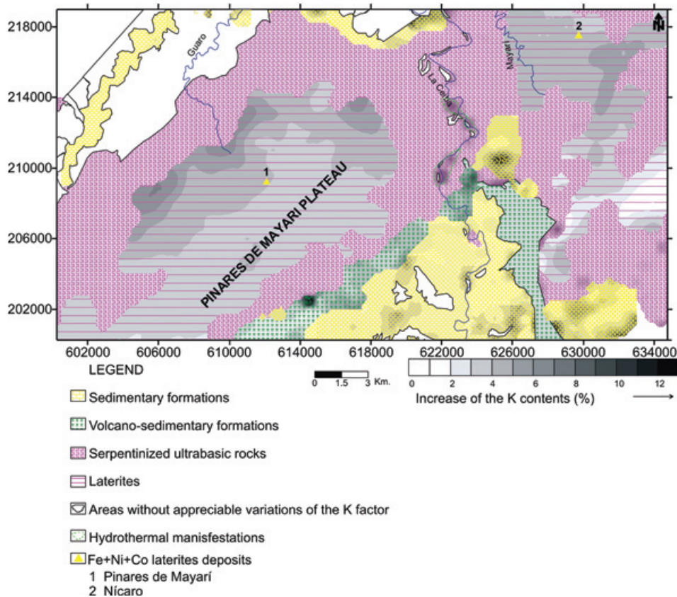
Fig. 11. Variations in the potassium (K) content of rocks of the Mayarí sector, according to K factor.
