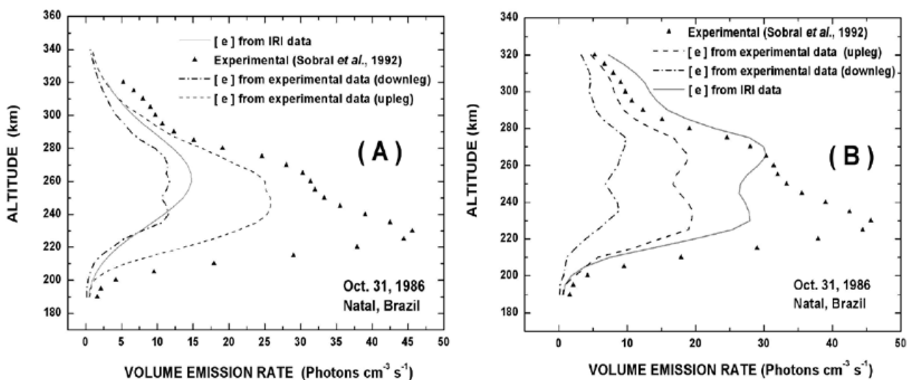
Fig. 3. Comparison between OI 630 nm red line volume emission rate profiles derived from the experiment carried out in October 31, 1986 (Sobral et al. , 1992) and calculated profiles. ( A ) The theoretical profiles with constant quantum yield f(1D) \sim 1.2 (Link and Cogger, 1988) were evaluated from experimental data of electron density (upleg and downleg) and IRI electron density data. ( B ) The theoretical profiles with height-dependent profile for f(1D) obtained from Sobral et al. (1992) were also evaluated from experimental data of electron density (upleg and downleg) and IRI electron density data.
