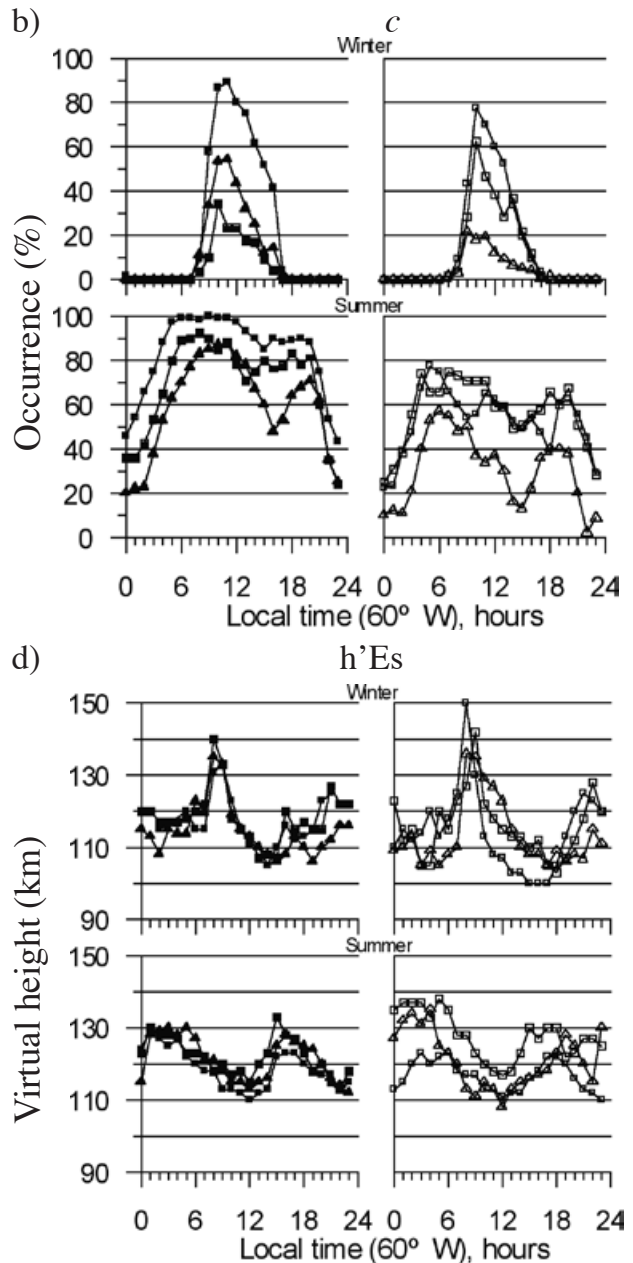
Es-type season occurrence and Es-characteristics season means at Argentine Island (65.2°S, 295.7°E) during years of low (filled symbols) and high (open symbols) solar activity level for solar cycles 21 (circles), 22 (squares) and 23 (triangles). (a) l -type, (b) c -type, (c) fbEs and (d) h'Es .
