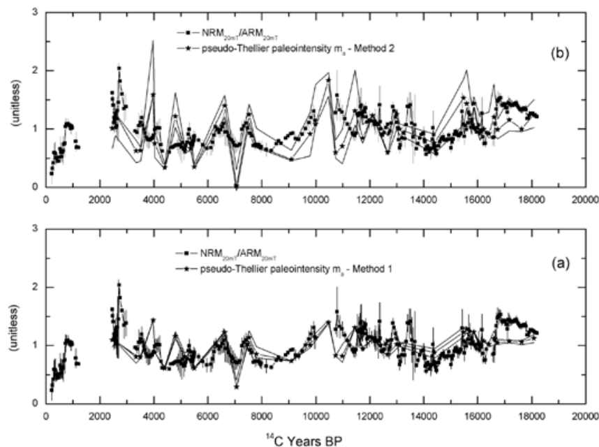
Fig. 5 (a). Comparison of ( · ) Relative paleointensity estimate using a conventional method: NRM_{20mT}/ARM_{20mT} vs. ^{14}C years BP (Gogorza et al. , 2006) with Pseudo-Thellier paleointensity estimate m_a . (★) is the best-fit slope m_a through at least four successive data points from NRM_{left} versus ARM_{gained} plot for each sample; solid lines indicate upper and lower limits of 90 per cent confidence level of slope m_a determined by jackknife resampling using Method 1. (b) same as (a) but for Method 2.
