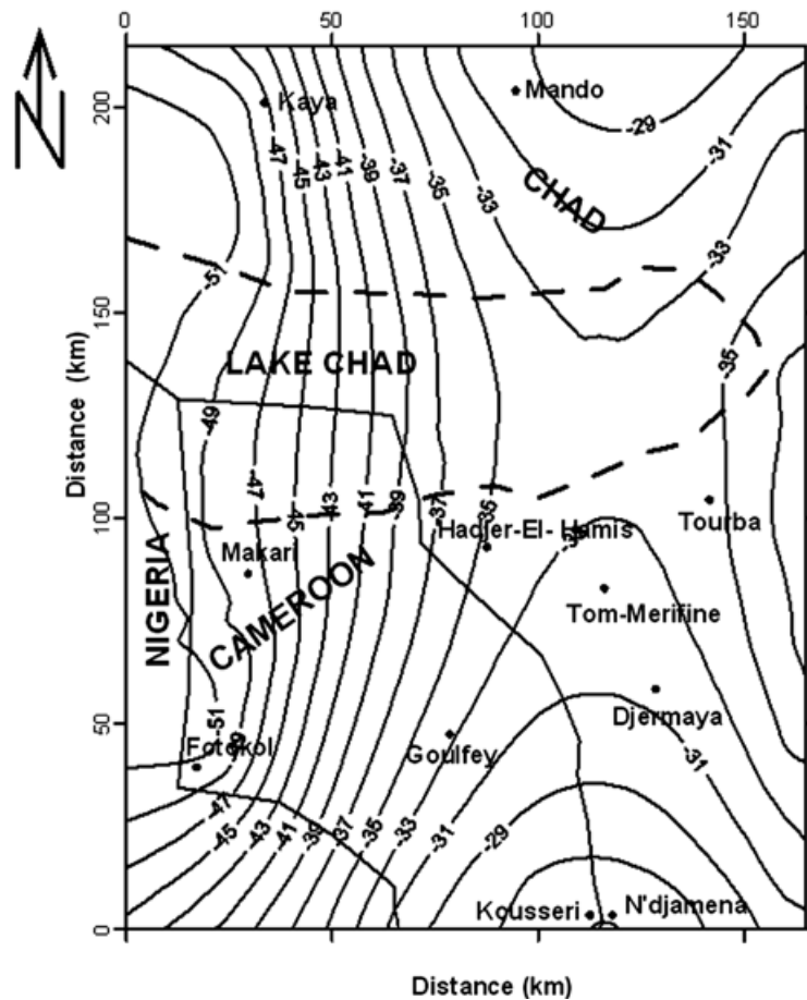
Fig. 3. Regional gravity anomaly map of the study area (Chad-Cameroon).
