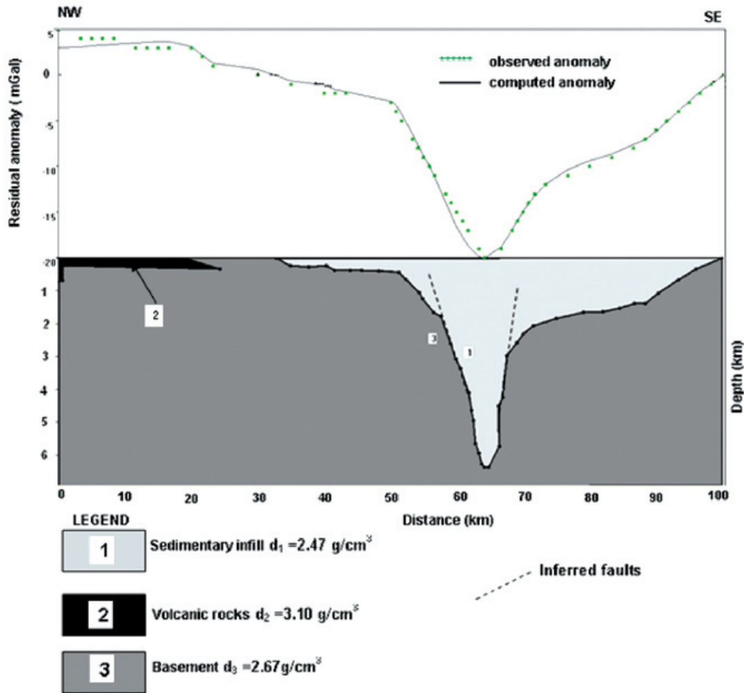
Fig. 6c. Interpreted model of profile P3 over Tourba.
