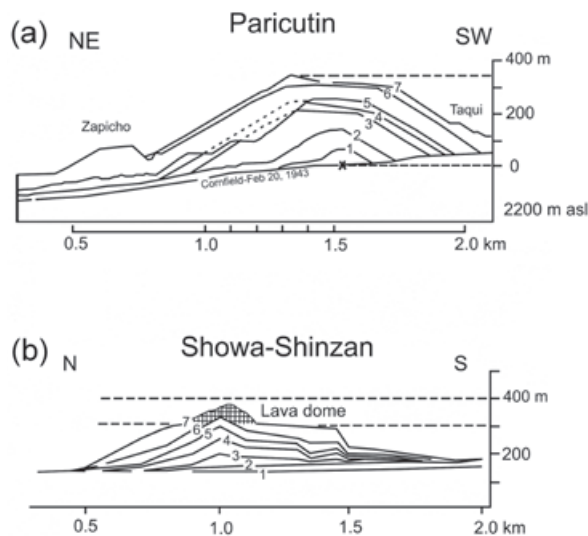
Figure 2. (a) Growth profile of Paricutin (UNAM-IGEOL, 1945, Appendix). (1): Feb. 23, 1943, (7): Feb. 20, 1944. (b) Growth profile of lava dome Showa-shinzan, Japan (Yokoyama, 2004), (1): Apr. 27, 1944, (7): May 18, 1945.
