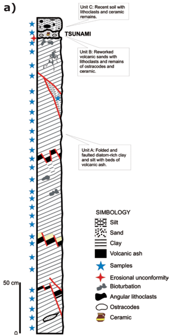
Figure 7a. Lithological column of western wall, trench 6 and photograph of wall.
