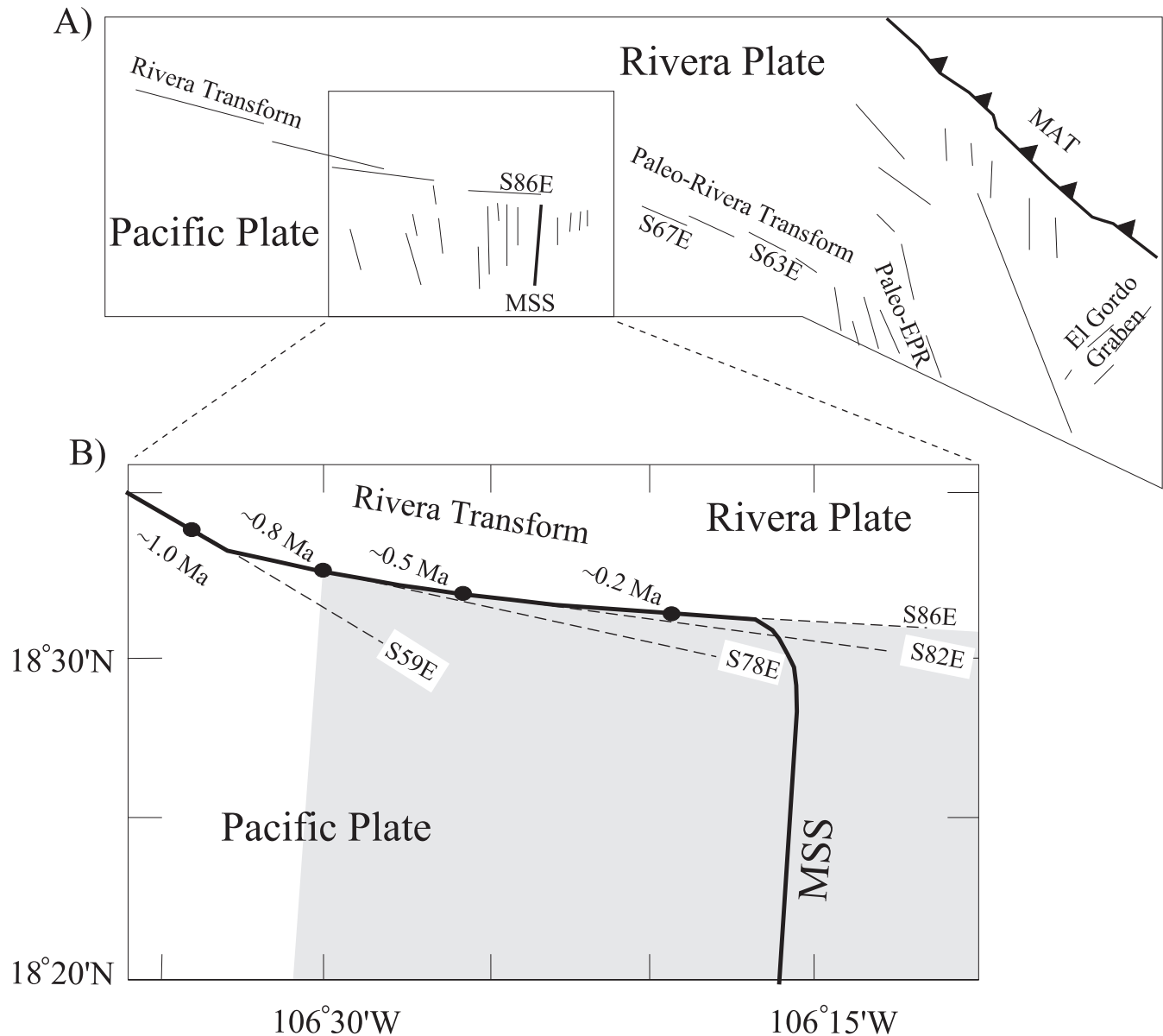
Fig. 3. Line drawing representation of the orientations of the morphologic features at the eastern end of the Rivera transform. Illustrated are the westward relocation of the EPR and the recent counterclockwise reorientation of the Rivera transform as it approaches the Moctezuma spreading segment (MSS). Labels on dashed lines are the direction of the tangents to the Rivera transform at the positions marked by the solid circles. Ages adjacent to solid circles represent the ages of the Pacific Plate immediately south of the transform. These ages were determined from magnetic anomaly lineations and by assuming a constant spreading rate at the MSS since 0.78 Ma. Original bathymetric maps from which the line drawing interpretation was determined are from Bourgois et al. [1988] and Michaud et al. [1996].
