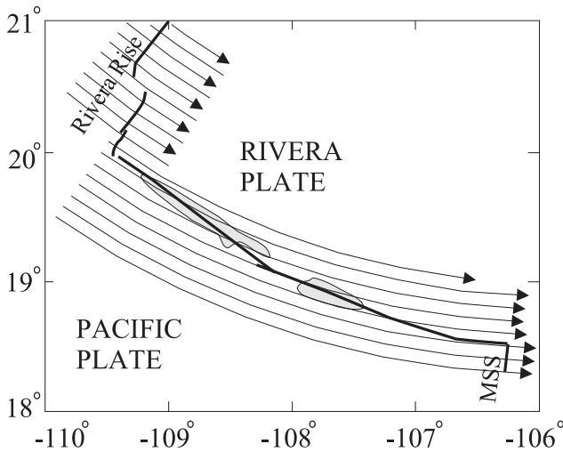
Fig. 7. Direction of motion of the Rivera plate relative to a fixed Pacific plate along the Rivera transform. The Rivera transform, MSS and Rivera Rise are marked by bold lines. The direction of motion of the Rivera plate relative to a fixed Pacific plate as predicted from the newly determined Rivera-Pacific Euler pole is marked by curved arrows. Shaded areas delineate the location of the deep bathymetric trough (depths > 4250 meters) associated with the Rivera transform (after Michaud et al. [1997]).
