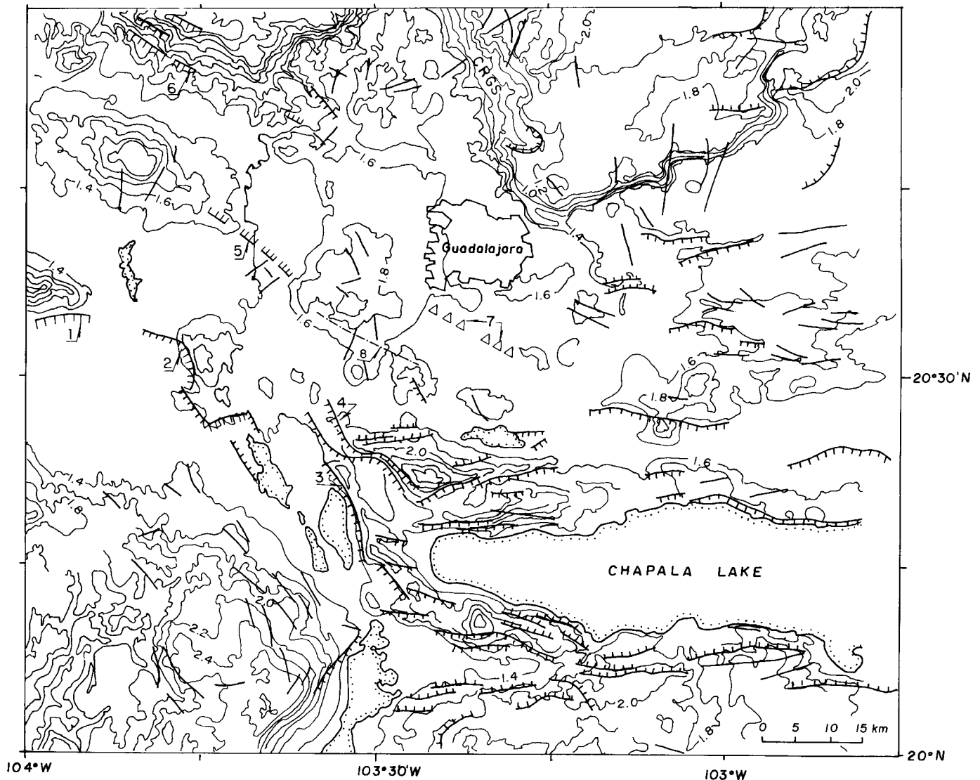
Fig. 3. Topography and structural setting of the study area. Contours are given in km. Main normal faults are indicated by continuous hatched lines. 1: Ameca fault; 2: Ahuiscalco fault; 3: San Marcos fault; 4: Bola de Viejo fault; 5: southward prolongation of Plan de Barrancas fault; 6: Santa Rosa fault; 7: southern Guadalajara volcanic chain system; 8: fault inferred by Alatorre-Zamora and Campos-Enríquez (1991).
