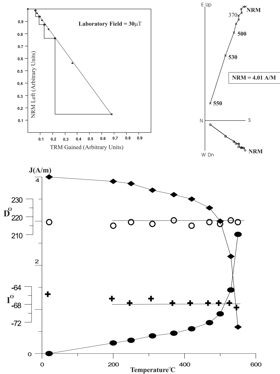
Fig. 4. Example of Thellier paleointensity determination for a hyaloclastite (Goguitchaichvili et al. , 1999b). Upper part NRM-TRM plot and associated Zijderveld diagram; the numbers refer to temperatures in °C, o projection into the vertical plane, x projection on the horizontal plane; Lower part, alternative presentation with incorporation of TRM acquisition curve. (+) Inclination, (o) Declination, (♦) NRM left, (●) TRM gained.
