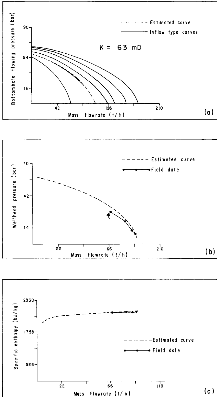
Fig. 6. Permeability diagnostic for Well Az-33 [Table 3]. (a) Overlap of well inflow curve with the inflow type-curves corresponding to T_0 = 275^\circ\text{C} , P_0 = 68.56 bar and Corey-type relative permeability. Inferred absolute permeability: 63 mD; (b) Estimated output curve of mass productivity, associated to the well inflow curve; (c) Estimated output curve of thermal productivity, associated to the well inflow curve.
