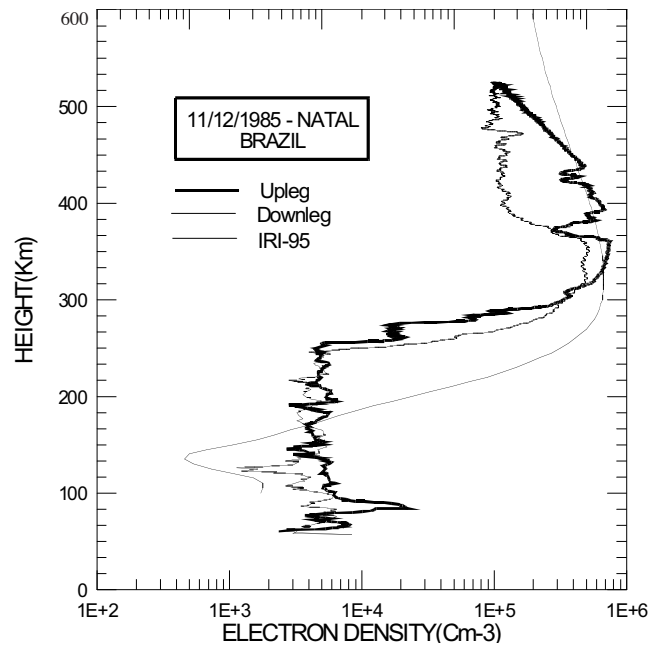
Fig. 2. Upleg n_e profiles from the LP and HFC measurements made on 11-th December, 1985 compared with the IRI-95 profile.
