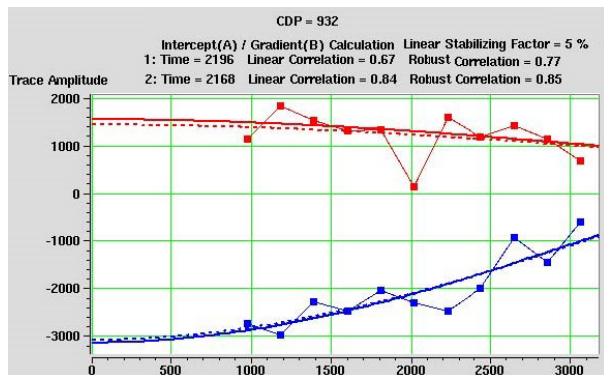
Figure 13. Sawan-7 AVO analysis at 2168 ms. The extracted amplitude values at the trough are shown in blue and at peak are shown in red respectively. The extrapolated zero offset amplitude value is just below -3000.
