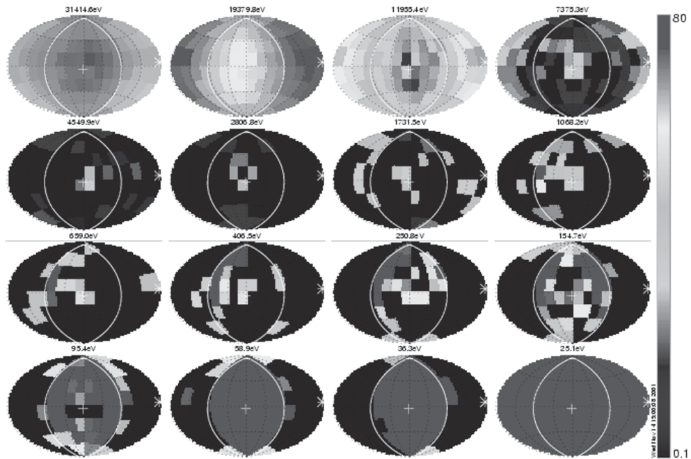
Fig. 5. Global distributions of H + and O + measured by Rumba on March 31, 2001 from 8:15-8:20 UT.
