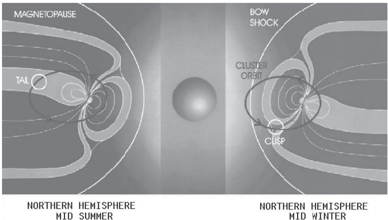
Fig. 1. The Cluster orbit.
