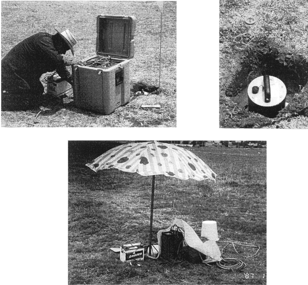
Fig. 2. Used equipment. Digitalizer and recording equipment REFTEK, GURALP sensor and a view of a station.
