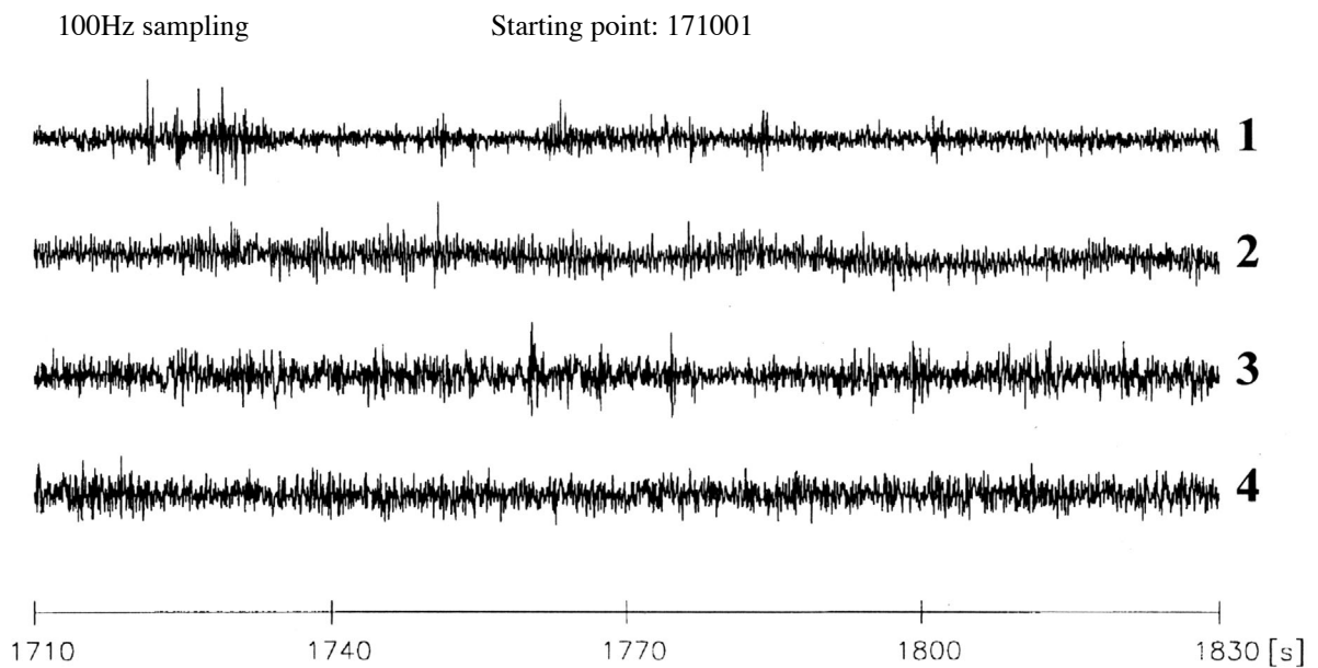
Fig. 3. Example of microtremor recording from CU array. The numbers correspond to the stations from one to four, from top to bottom respectively.
