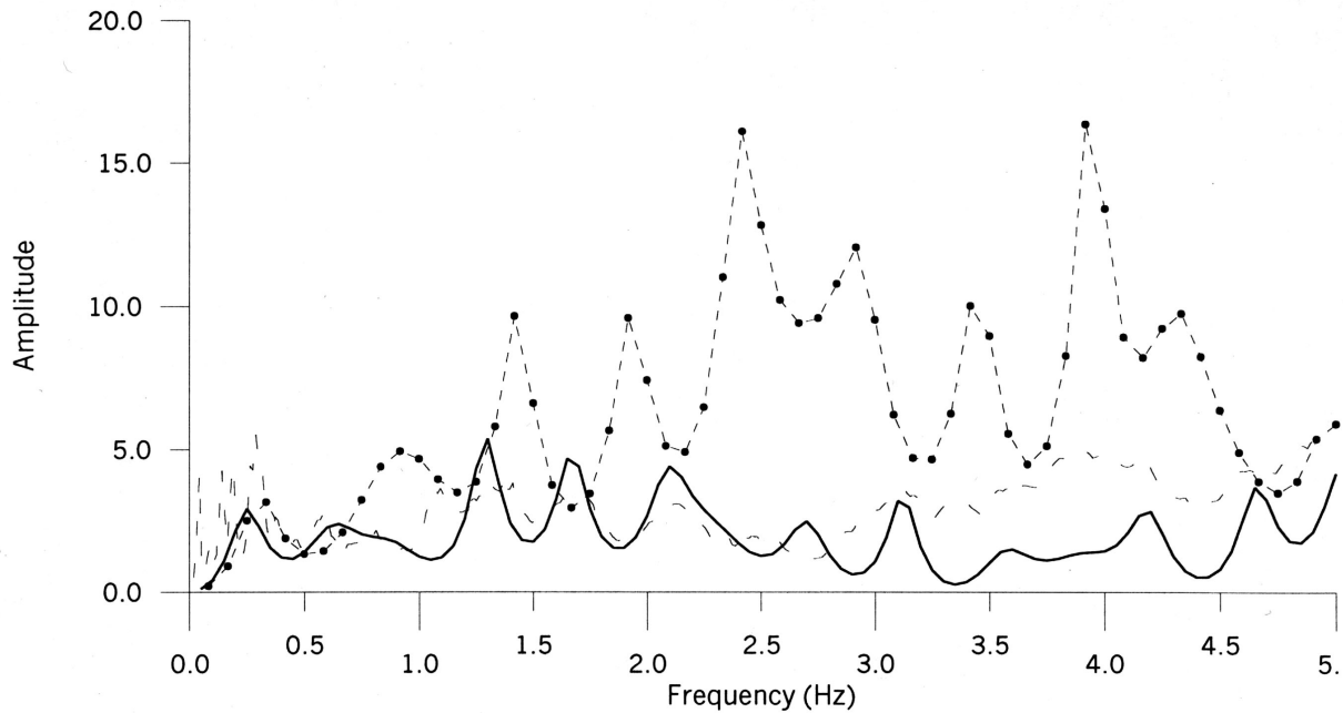
Fig. 10. Comparison between transfer functions for the model obtained in this work with SPAC method (continuous line); for the model by Kagawa et al. (1996) using F-K method; and empirical transfer function obtained by Montalvo et al. (2002) using spectral ratios for the Tehuacan earthquake (June 15, 1999).
