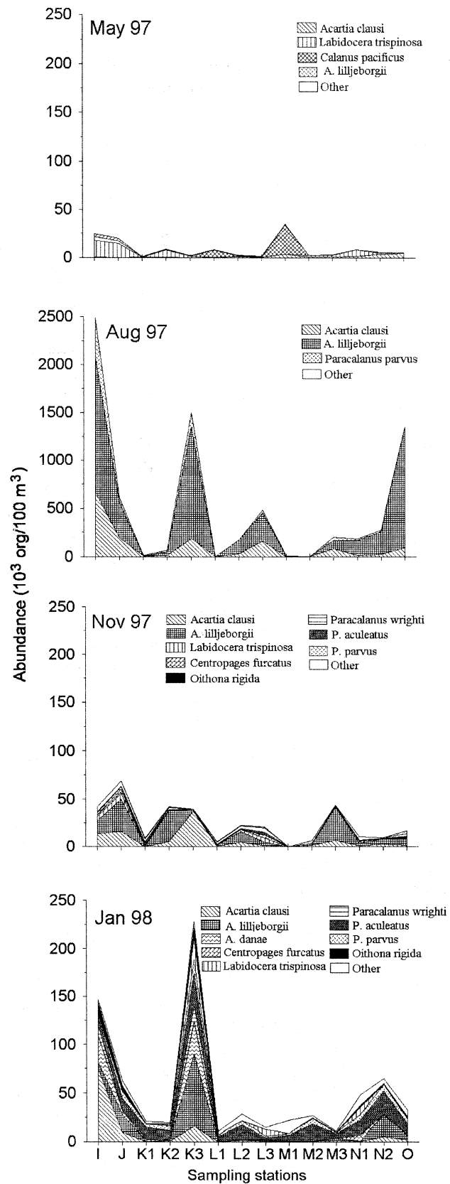
Fig. 3. Copepod community structure (abundance org/100 m 3 ) during the 1997-98 El Niño in Bahía Magdalena. Graphs show species accounting for 90% of total abundance.
