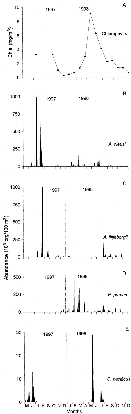
Fig. 4. A) Monthly mean chlorophyll a concentration ( \text{mg}/\text{m}^3 ) at 5 meters depth (solid line) and (B - E) size abundance of four copepod species, during 1997-98 in Bahía Magdalena.
