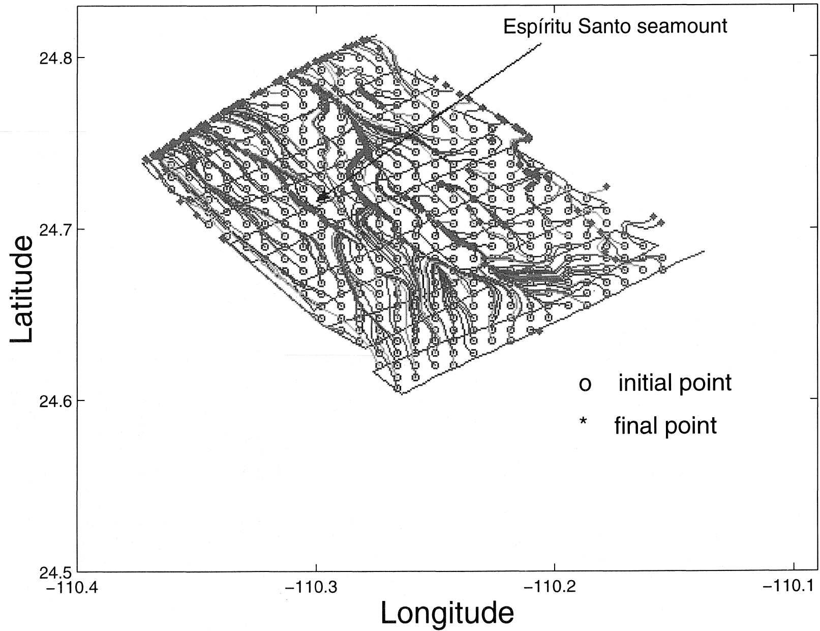
Fig. 9. Lagrangian trajectories of regularly spaced particles in the surface flow field during a 12-hour simulation, assuming stationary flow.
