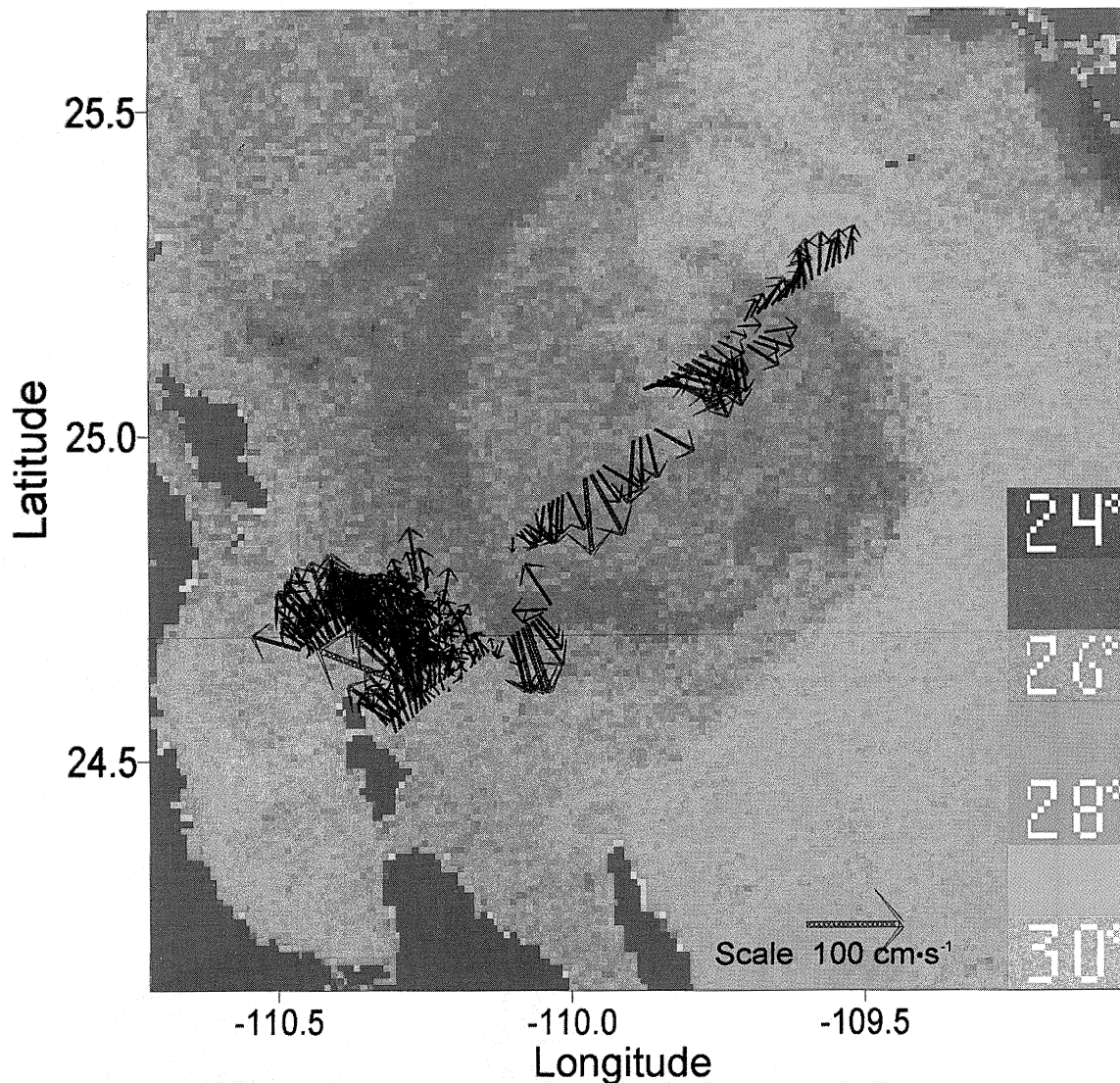
Fig. 2. Satellite image of 17 November 1995 showing temperatures in false color. Surface currents from the ADCP survey of 24 November 1997 are shown superimposed.
