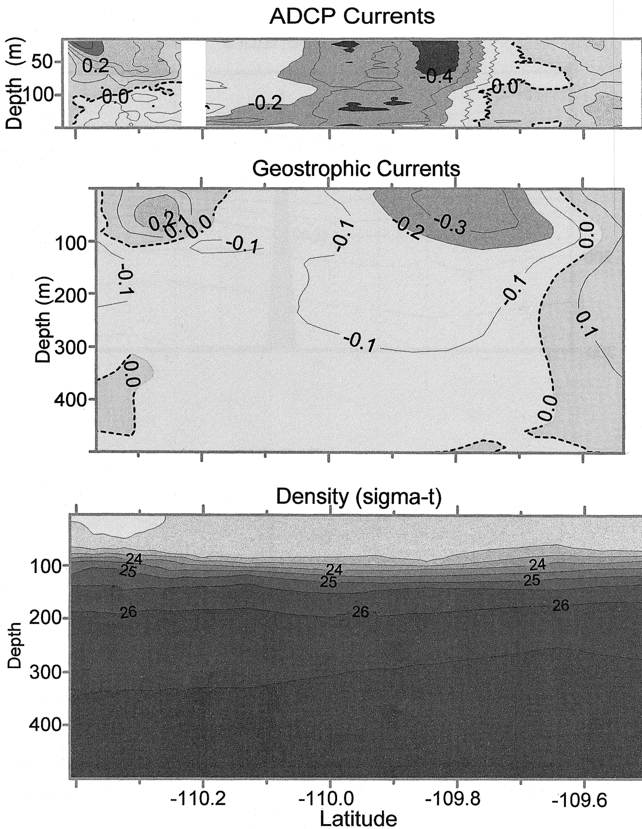
Fig. 6. Large scale vertical behavior of (all stations in Line H): a) ADCP current component perpendicular to the line; b) geostrophic currents; c) density section.
