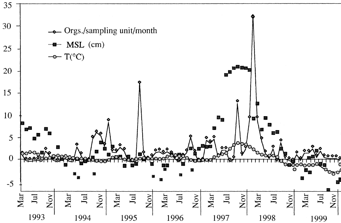
Fig. 7. Relationship between juvenile spiny lobster settlement, sea surface temperature and mean sea level anomalies.
