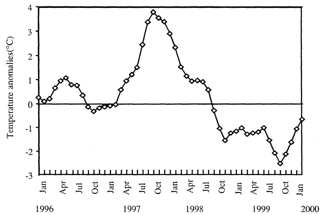
Fig. 2. Sea surface temperature anomalies. (From COADS / NOAA at 27° N, 114° W, January 1996 to January 2000.
