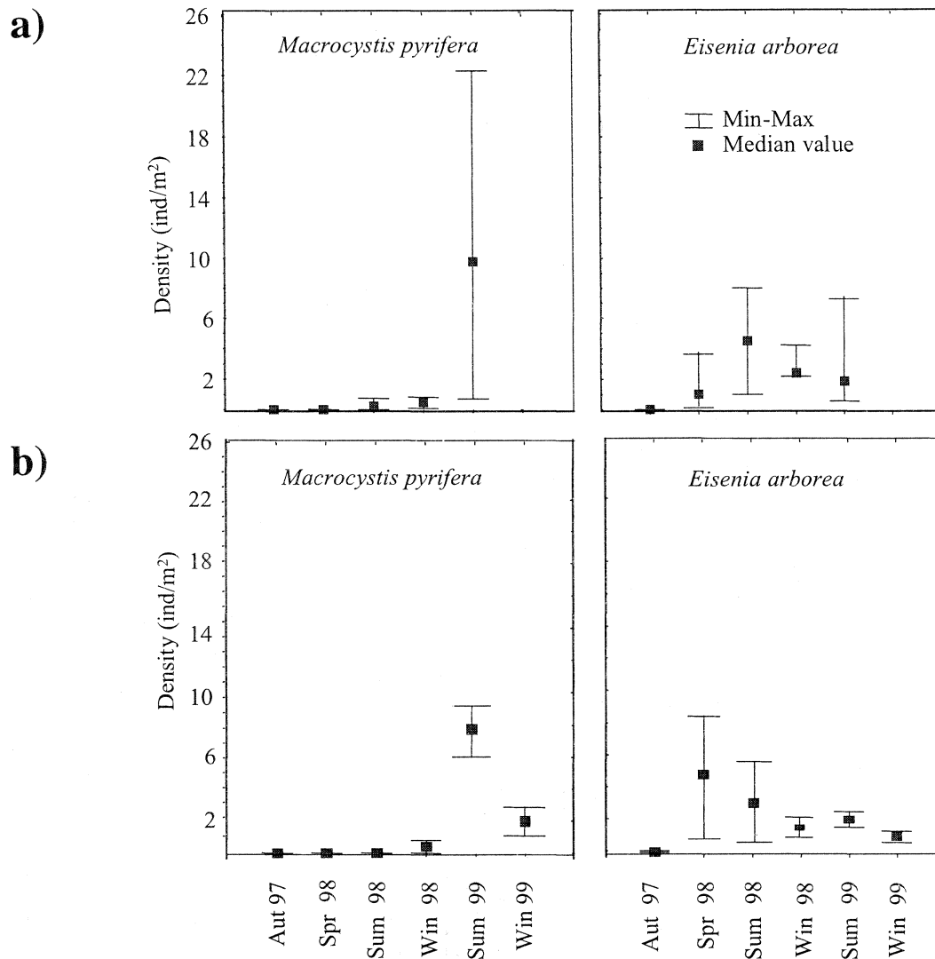
Fig. 6. Differential recruitment lag after El Niño in densities of Macrocyctis pyrifera and Eisenia arborea a) Los Morros, b) Clam Bay.
