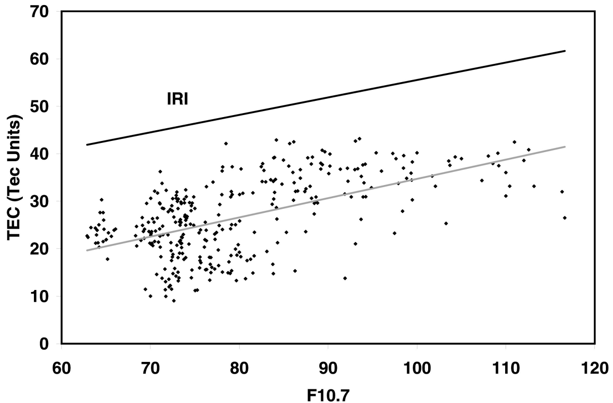
Fig. 6. TEC dependence on solar flux ( 62 < F10.7 < 116 flux units), at 1700 UT, maximum diurnal peak, for 1997. The upper straight line represents IRI-95 predictions.
