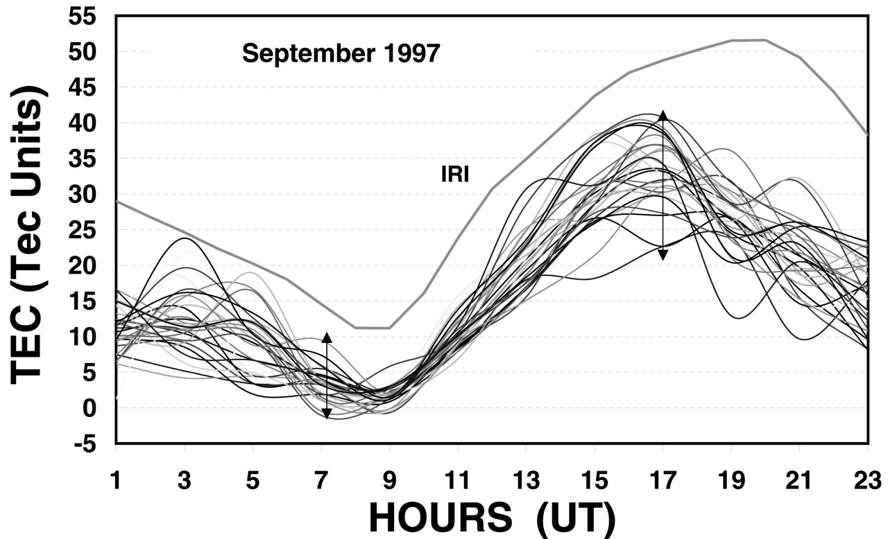
Fig. 3. Superposition of the diurnal plots obtained in September, 1997 (28 days available). The maximum dispersion of plots is shown as a bar at diurnal TEC peak.
