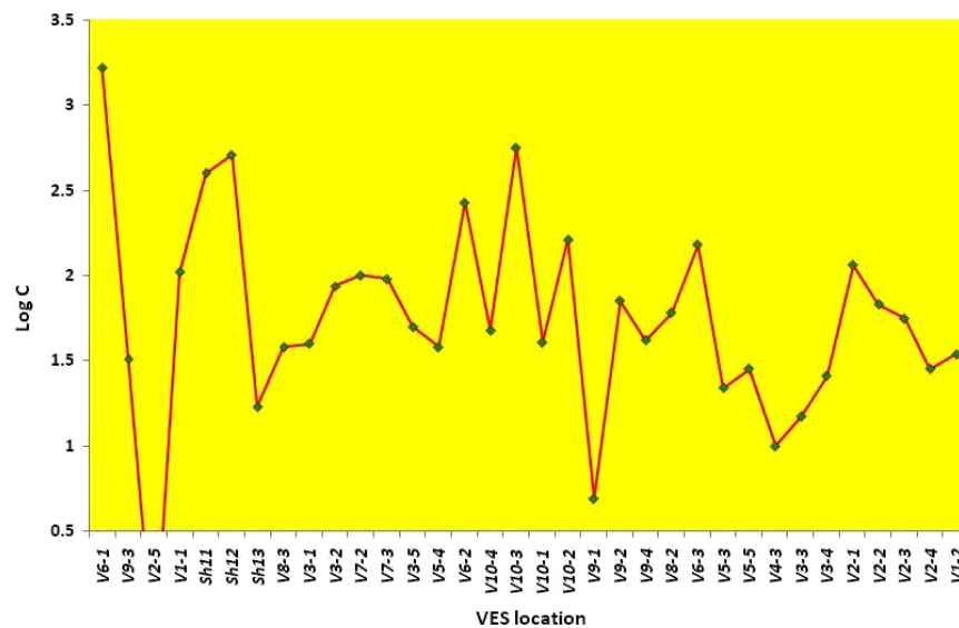
Figure 9. Variation of \log C with the thirty-four VES location points in the study area.
