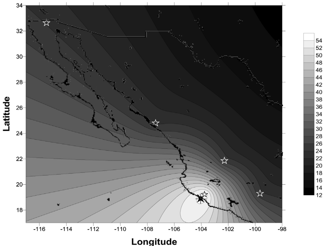
Fig. 6. Spatial distribution of \Delta\text{TEC} obtained from the data of INEGI GPS receivers network for 1010 LT 18 of January 2003.
